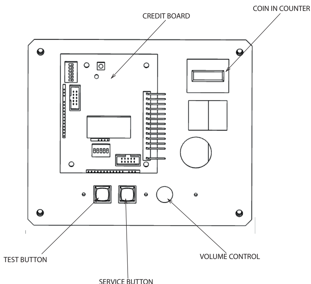
FIG. 9-1a Switch Unit
